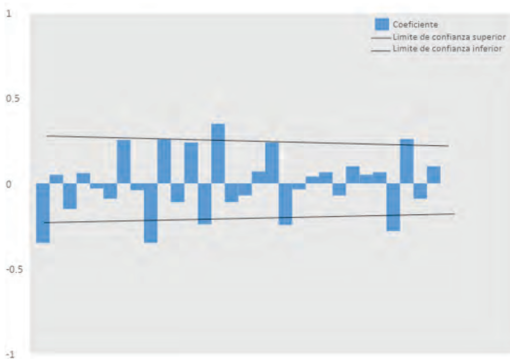
Graphic 1. Autocorrelation correlogram (ACF) estimated for the time series.
