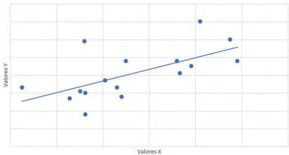
Graphic 1. Correlation scatter diagram between mPAP (x) and PSAP (y). mPAP: mean pulmonary artery pressure. PASP: pulmonary artery systolic pressure. r=0,647 , p=0,007
