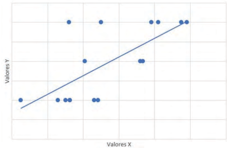
Graphic 4. Scatter diagram of correlation between mPAP (x) and probability for HAP (y). mPAP: mean pulmonary artery pressure. PAH: pulmonary arterial hypertension. r = 0,706 , p = 0,008
