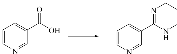
Scheme 1. Reagents and conditions: (a) \text{H}_3\text{BO}_3 , toluene (35%)
